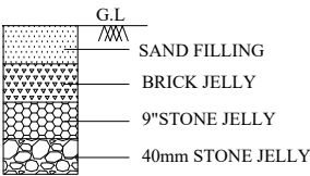
RAIN WATER HARVESTING RECHARGE PIT
