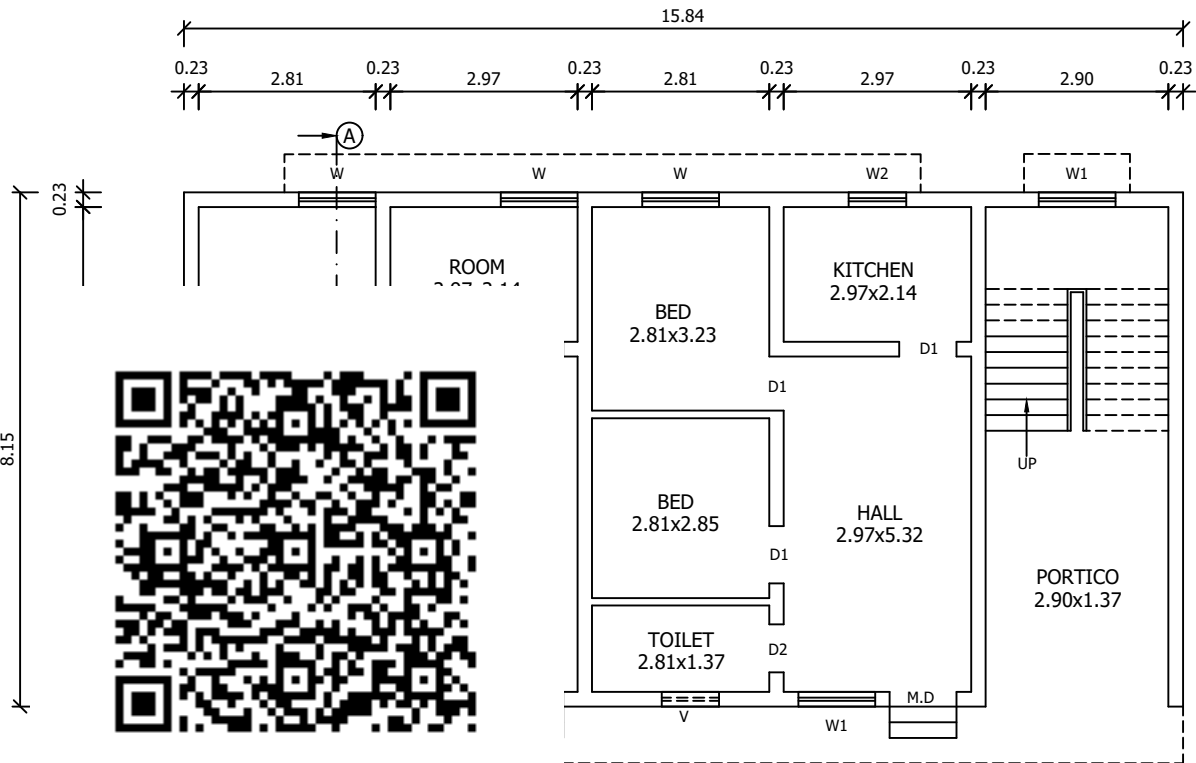
EXG. GROUND FLOOR PLAN
