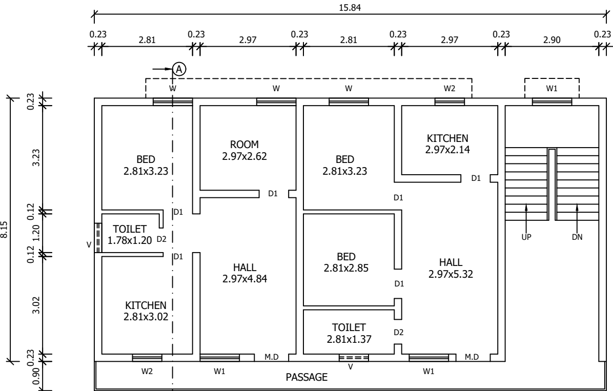
PRO. FIRST FLOOR PLAN
