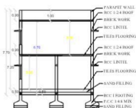
SECTION ON AB
