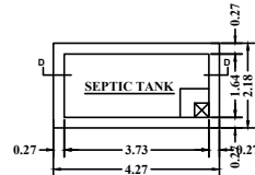
PLAN ON SEPTIC TANK . (NOT TO SCALE)
