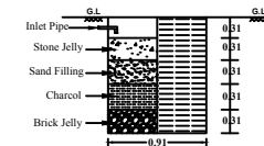
RAIN WATER HARVESTING DETAIL (NOT TO SCALE)
