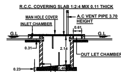
RAIN WATER HARVESTING DETAIL (NOT TO SCALE)
