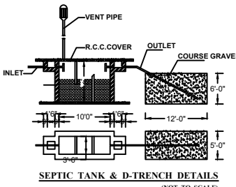
SEPTIC TANK & D-TRENCH DETAILS (NOT TO SCALE)
