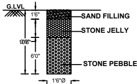
RAIN WATER HARVESTING PIT (NOT TO SCALE)
