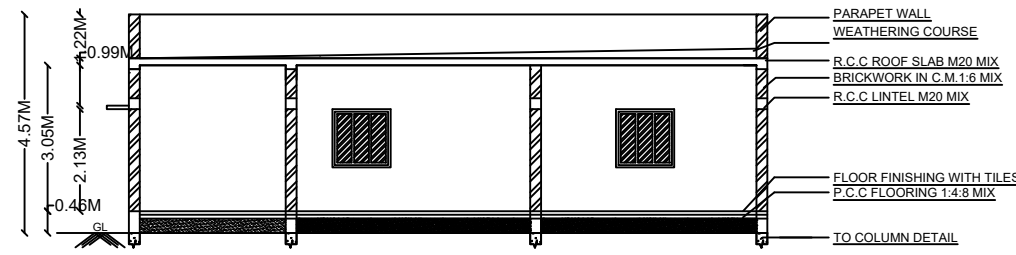
SECTION ON A-A
