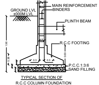
TYPICAL SECTION OF R.C.C COLUMN FOUNDATION
