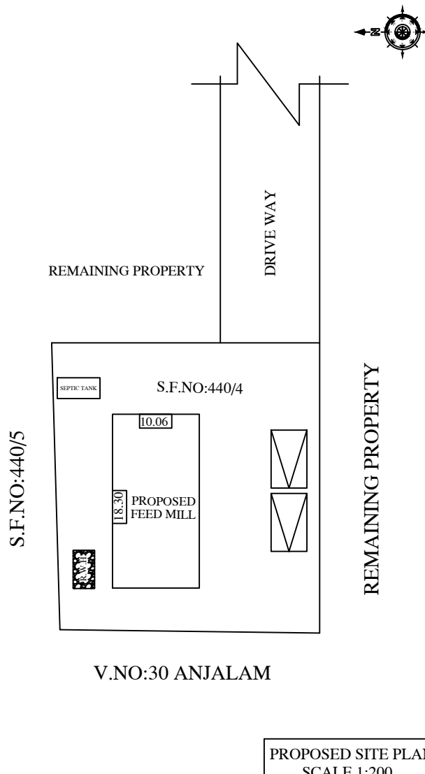
PROPOSED SITE PLAN SCALE 1:200
