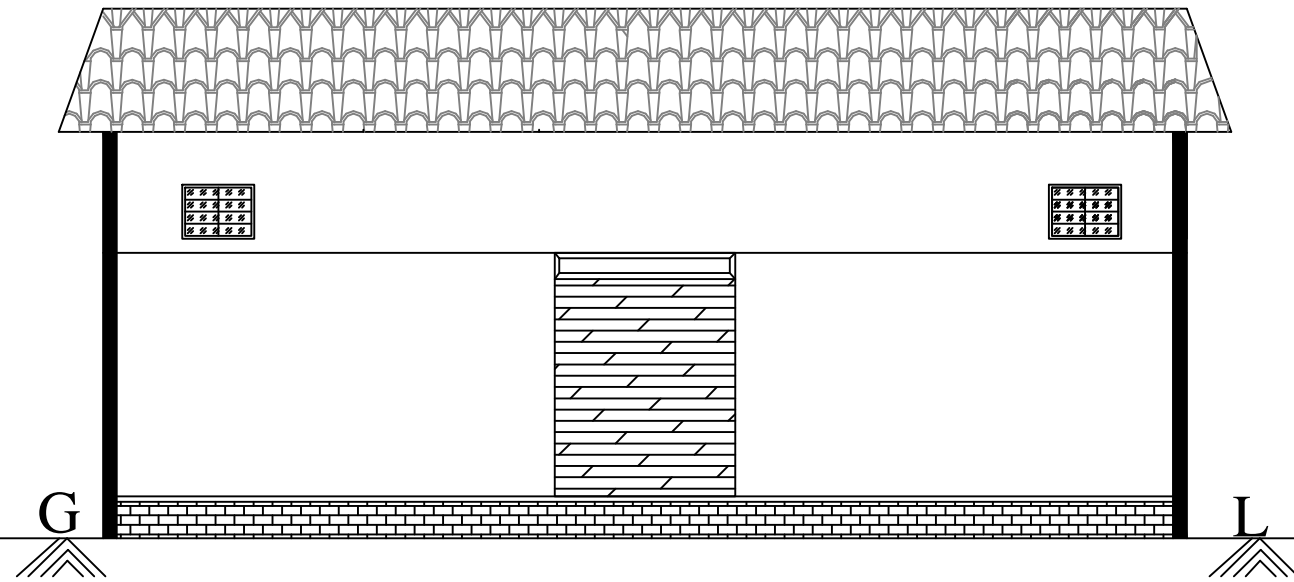
FRONT ELEVATION
