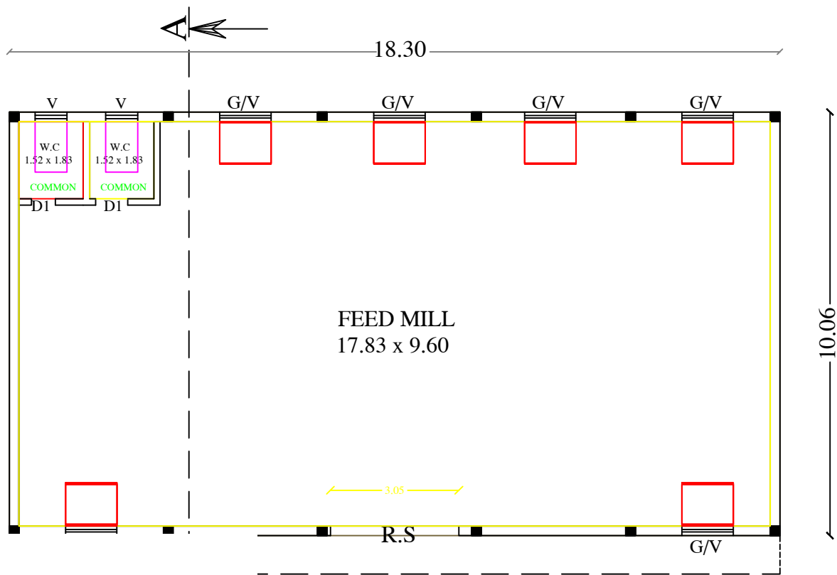
GROUND FLOOR-PLAN
