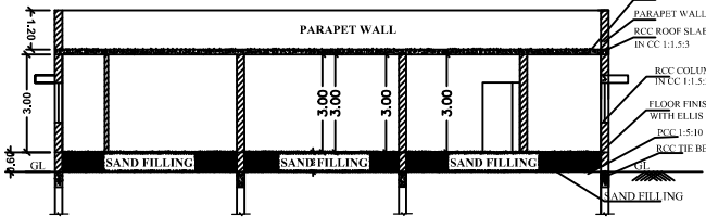
SECTION ON AA
