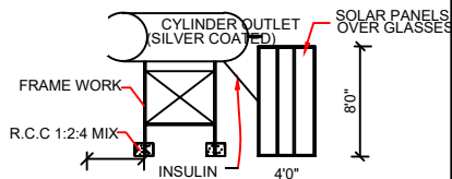
Waste Water Recycle Unit Not To Scale
