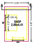
PRO.,GROUND FLOOR PLAN
