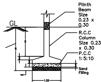
FOUNDATION DETAILS
