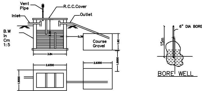
SEPTIC TANK & D-TRENCH DETAILS
