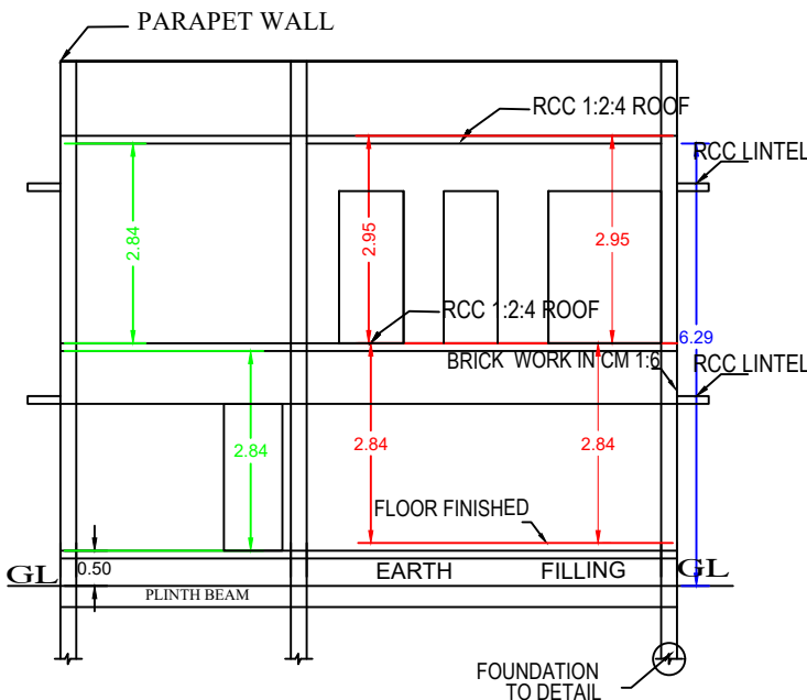
SECTION "A-B"
