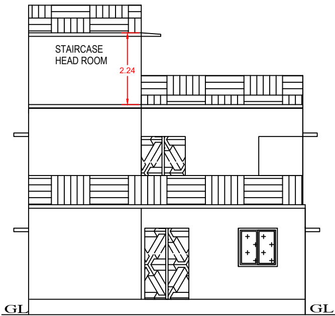
FRONT ELEVATION.
