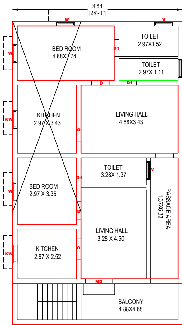
EXG.PRO. FIRST FLOOR PLAN.
