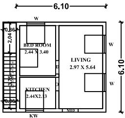
PRO.GROUND F
