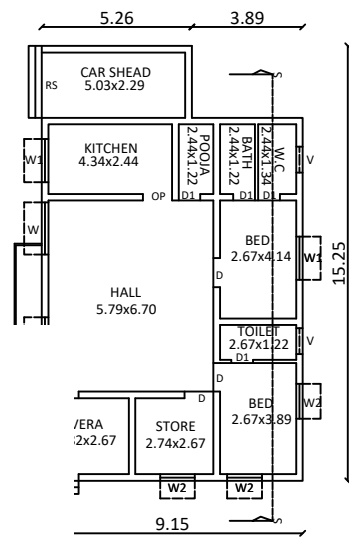
(EXISTING) GROUND FLOOR PLAN
