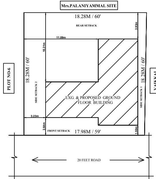
SITE PLAN
