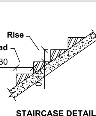
STAIRCASE DETAILS
