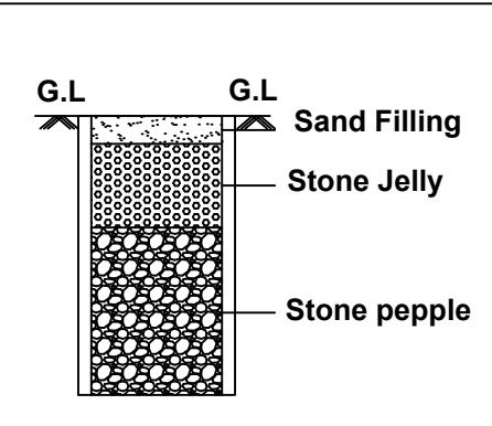
DETAILS OF RAIN WATER HARVESTING
