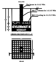
COLUMN AND FOUNDATION DETAILS
