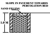
SECTION OF RAIN WATER PERCOLATION BED
