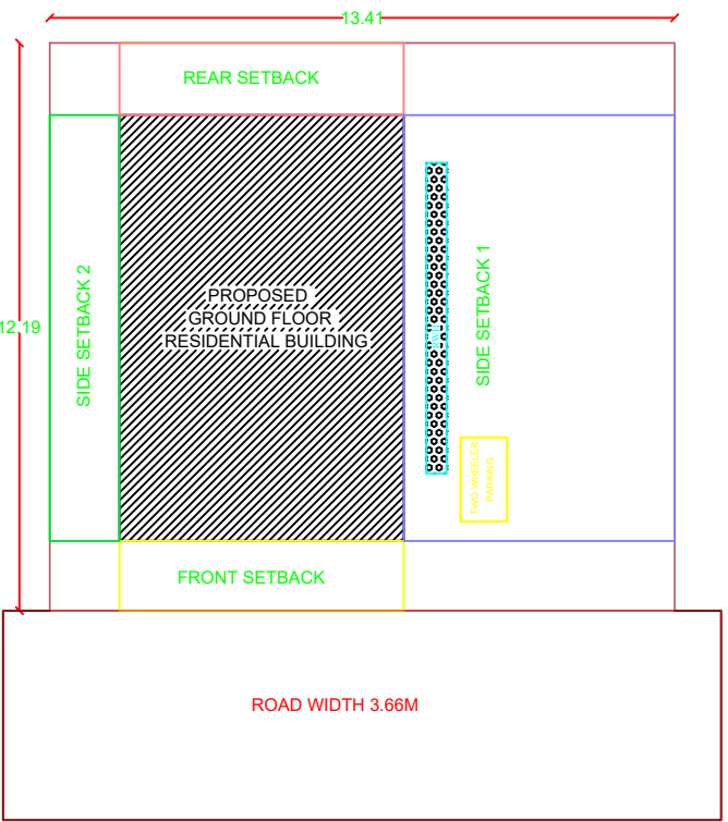
SITE PLAN
