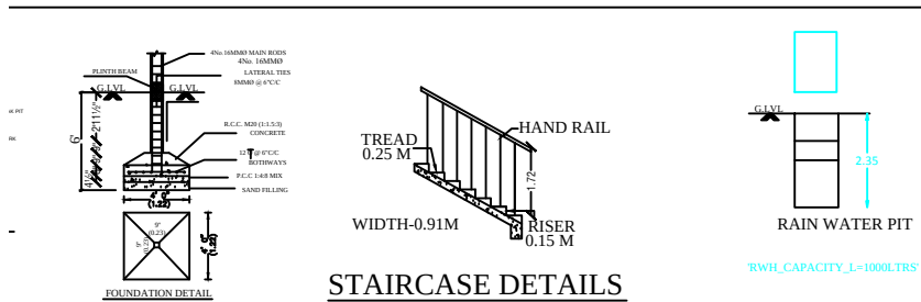
STAIRCASE DETAILS
