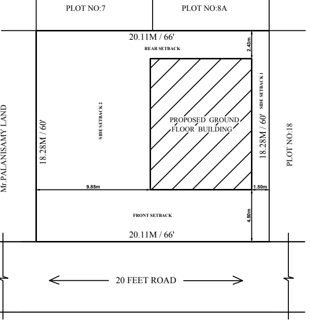
KEY PLAN
