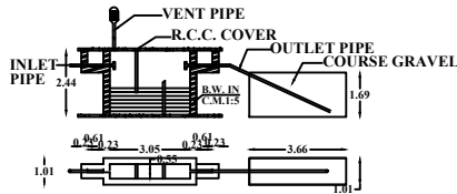
TANK & OF DISPERSION TRENCH DETAILS
