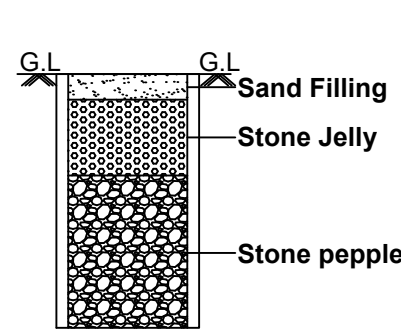
DETAILS OF RAIN WATER HARVESTING
