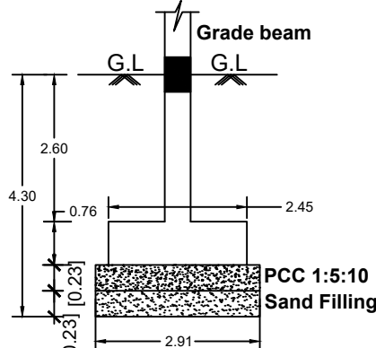
FOUNDATION DETAILS
