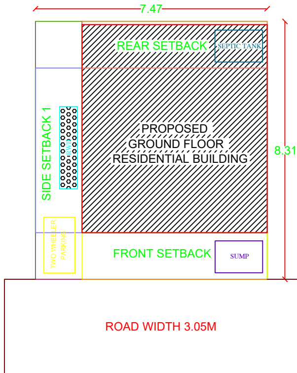
SITE PLAN
