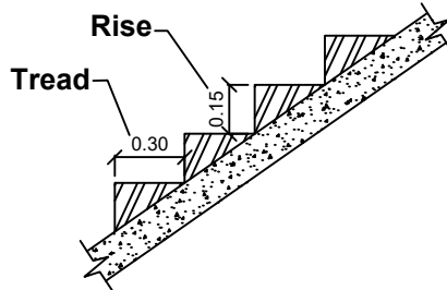
STAIRCASE DETAILS
