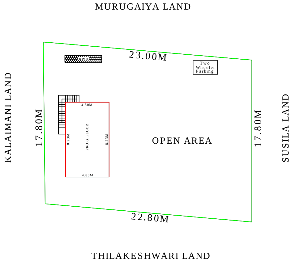
SITE PLAN
