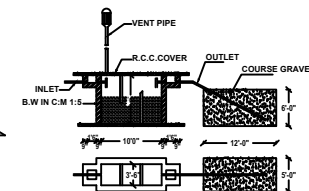
SEPTIC TANK & D-TRENCH DETAILS (NOT TO SCALE)
