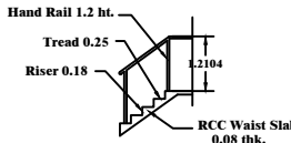
STAIRCASE DETAILS
