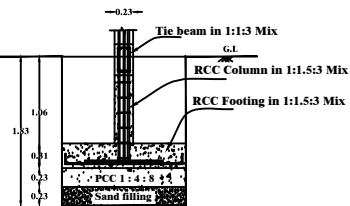
CROSS SECTION ON 'C - C'
