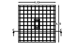
COLOUMN FOUNDATION DETAILS
