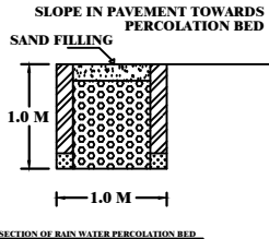
SECTION OF RAIN WATER PERCOLATION BED
