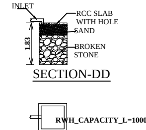
PLAN OF RWH
