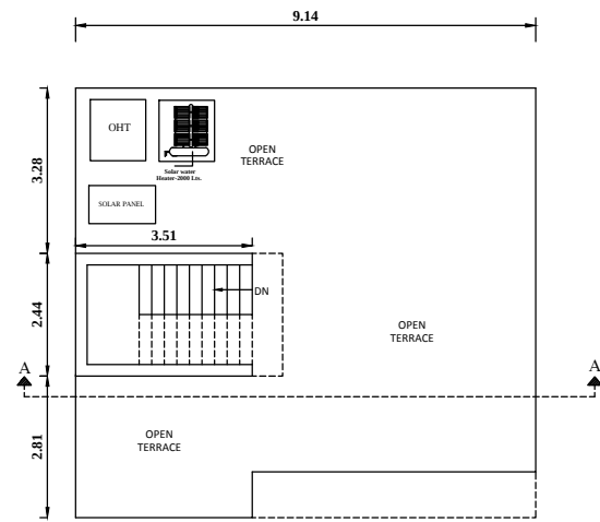
GROUND FLOOR ROOF PLAN
