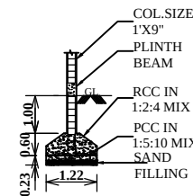
COLUMN DETAILS
