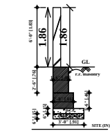
COMPOUND WALL
