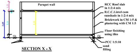
SECTION X - X
