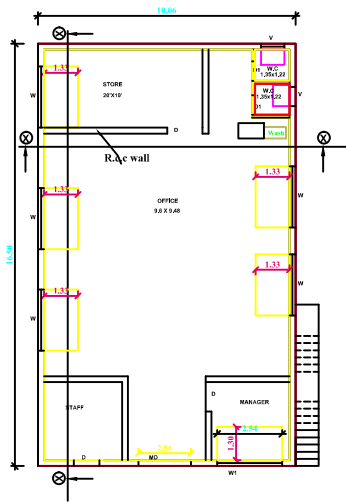
PLAN
