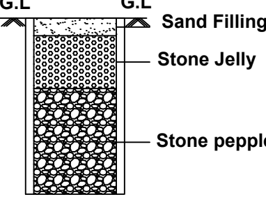
DETAILS OF RAIN WATER HARVESTING
