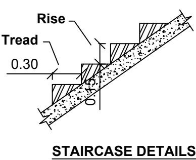
STAIRCASE DETAILS
