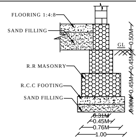
TYPICAL SECTION OF R.R MASONRY FOOTING DETAILS
