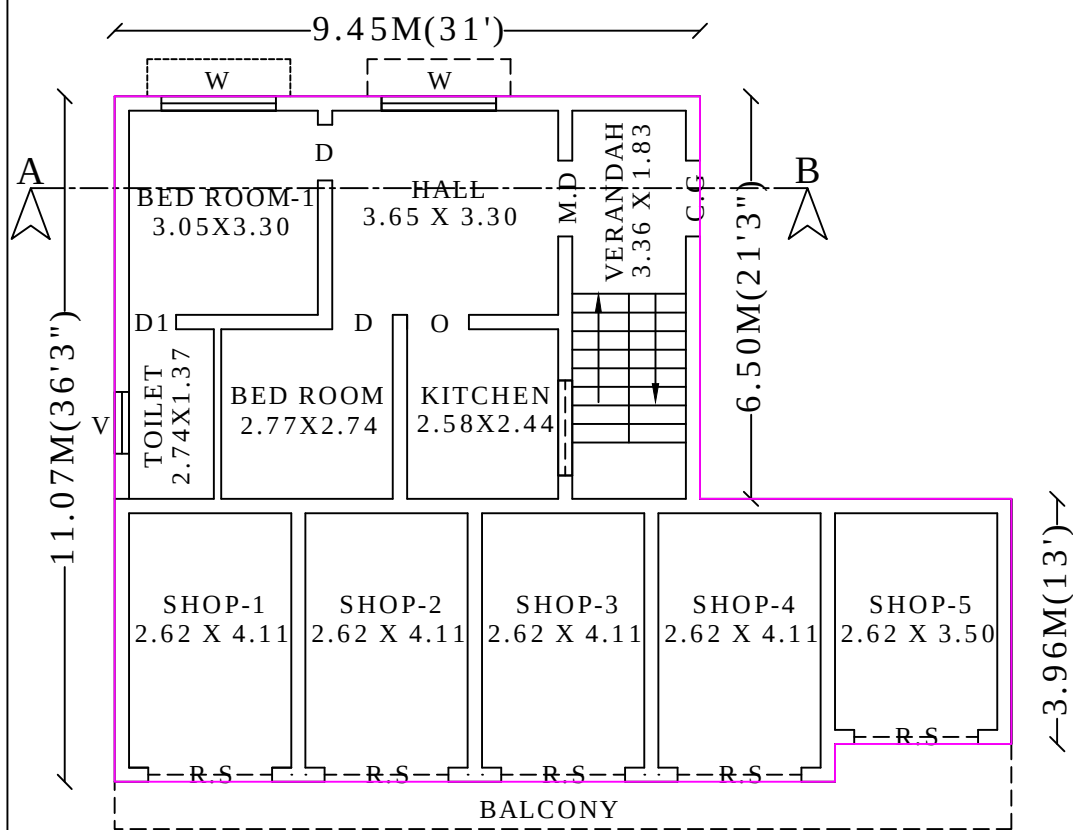
EXG.G.FLOOR HOUSE CUM SHOP PLAN (SOUTH FACING)
