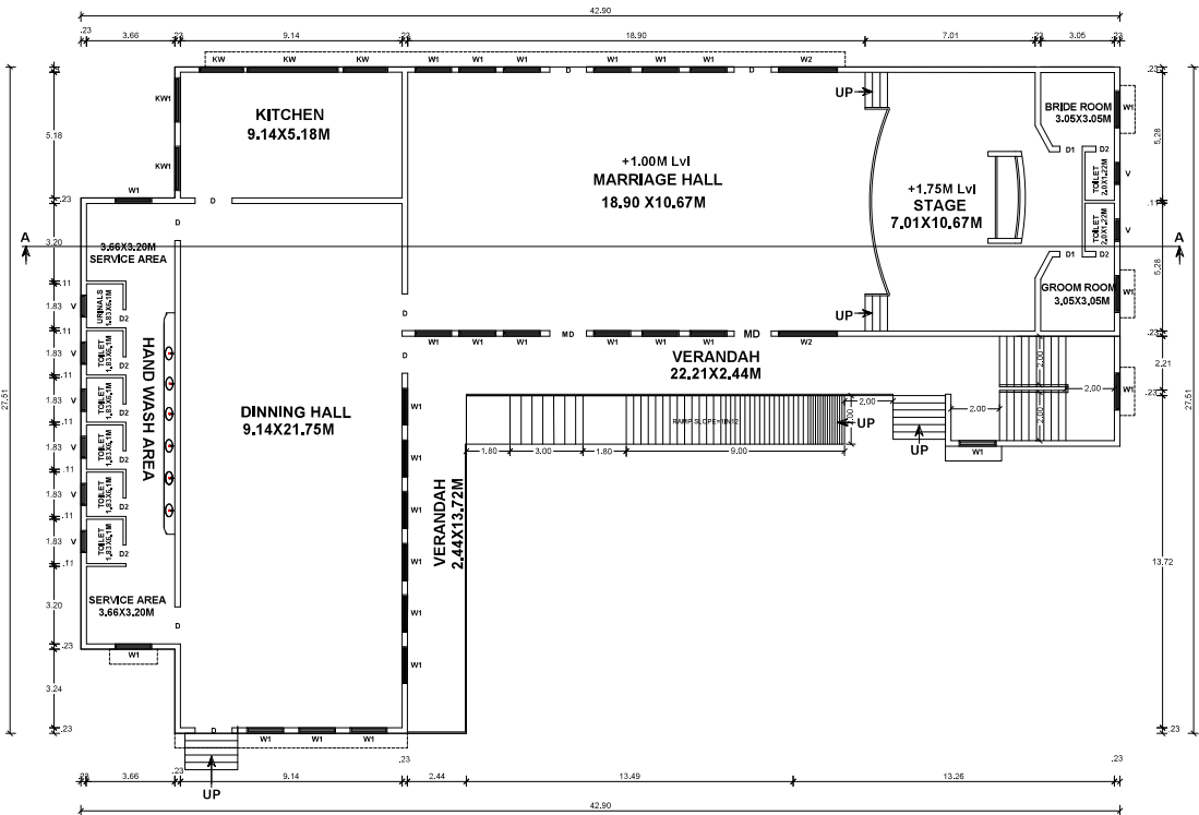
PROPOSED MARRIAGE HALL - GROUND FLOOR
