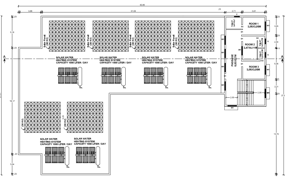
PROPOSED MARRIAGE HALL - FIRST FLOOR CUM TERRACE FLOOR PLAN
