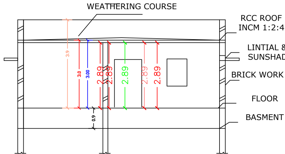
CROSS SECTION 'AB'
