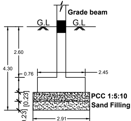
FOUNDATION DETAILS
