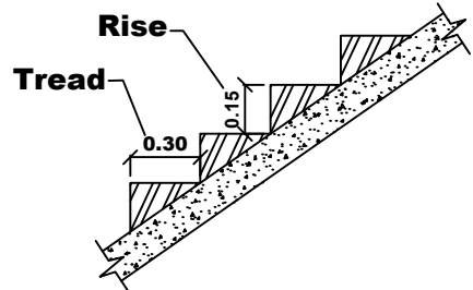
STAIRCASE DETAILS
