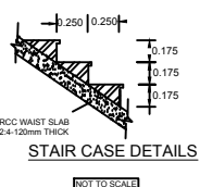
STAIR CASE DETAILS
