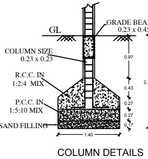
COLUMN DETAILS
