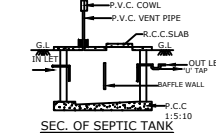
SEC. OF SEPTIC TANK
