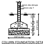
COLUMN FOUNDATION DETAIL
