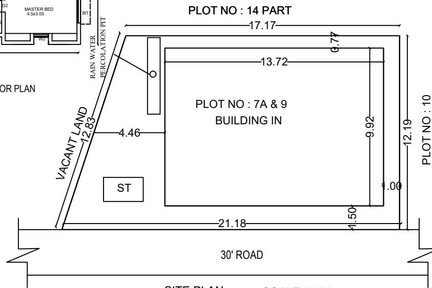
SCALE 1:100
