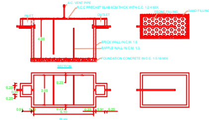
PLAN & SECTION OF SEPTIC TANK & DISPERSION TRENCH
