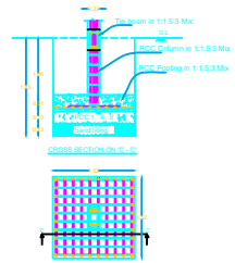
COLOUMN FOUNDATION DETAILS - A
