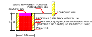
SECTION OF RAIN WATER PERCOLATION BED
