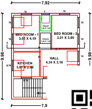
FLOOR- ( PRO.GROUN
