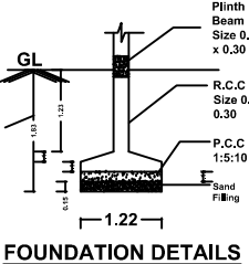
FOUNDATION DETAILS
