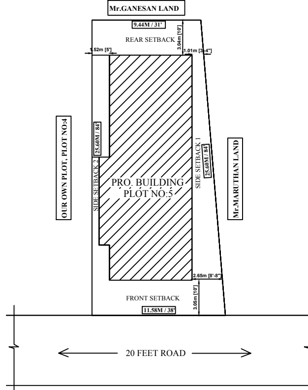
SITE PLAN
