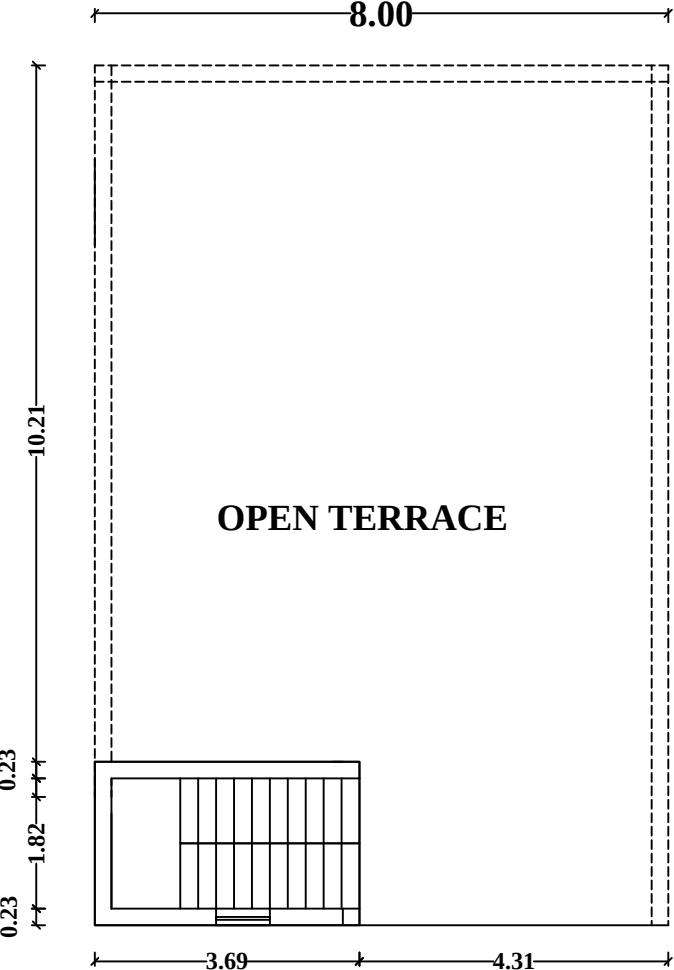
FLOOR-1 PRO.TERRACE PLAN
