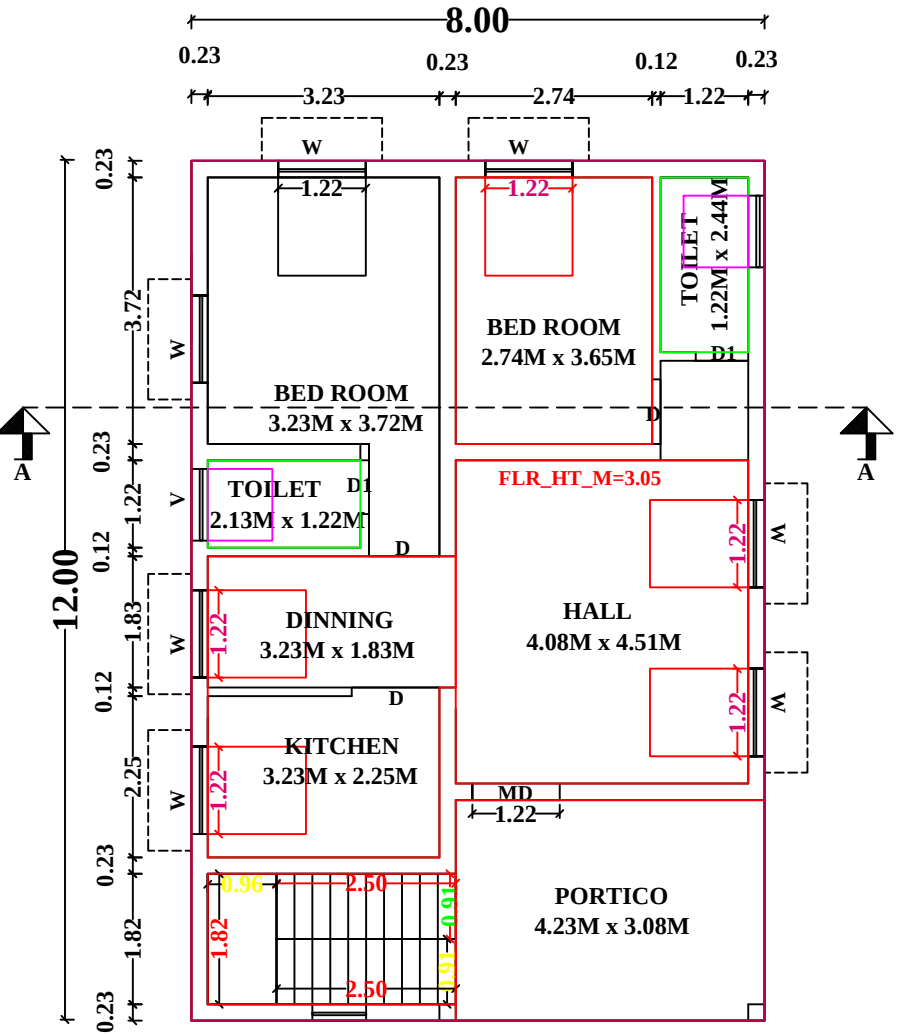
FLOOR-GROUND PRO.GROUND FLOOR PLAN
