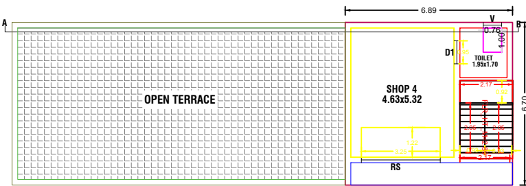
PRO., FIRST FLOOR PLAN
