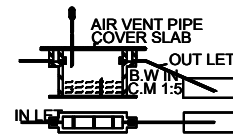
DETAILS OF SEPTIC TANK & D-TRENCH
