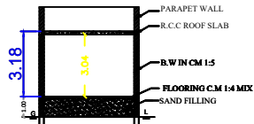
SECTION "AB"
