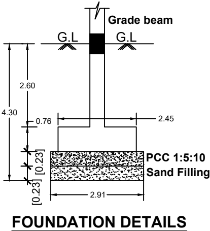
FOUNDATION DETAILS
