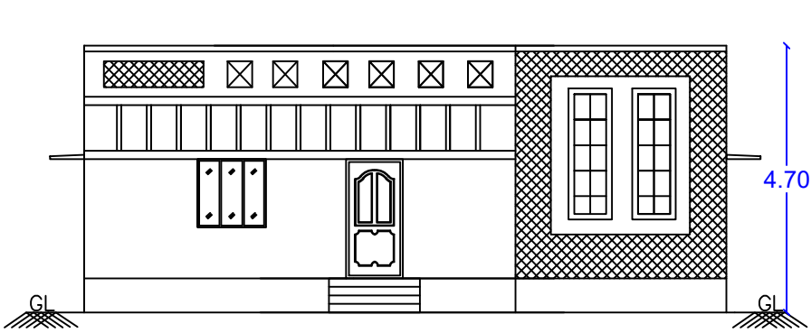
FRONT ELEVATION
