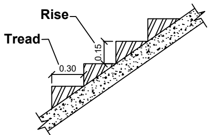
STAIRCASE DETAILS
