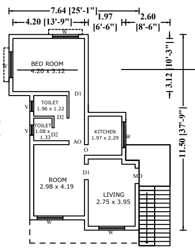
PRO. FIRST FLOOR PLAN
