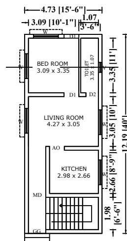
EXG.FIRST FLOOR PLAN
