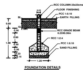
FOUNDATION DETAILS
