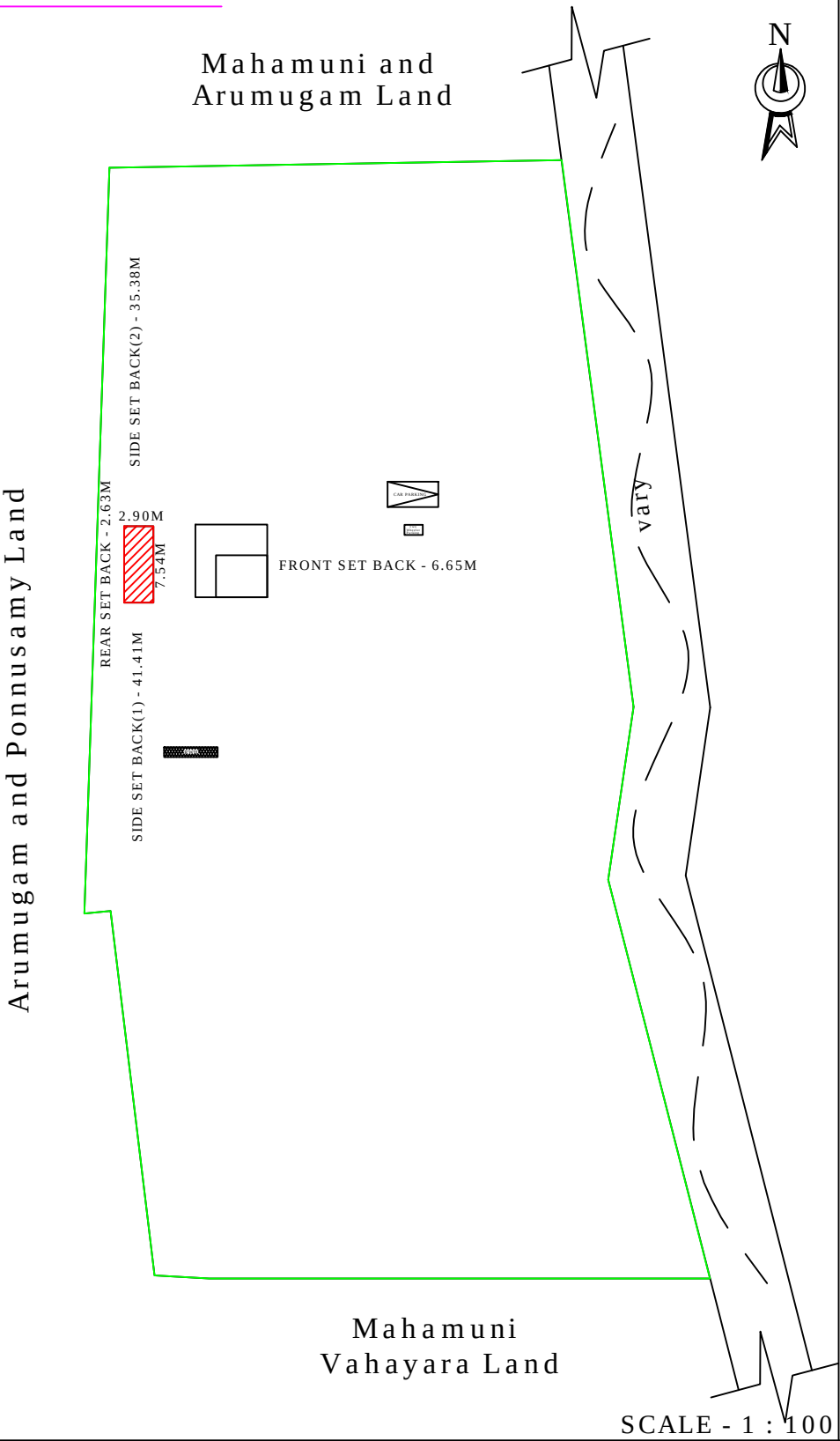
SITE PLAN
