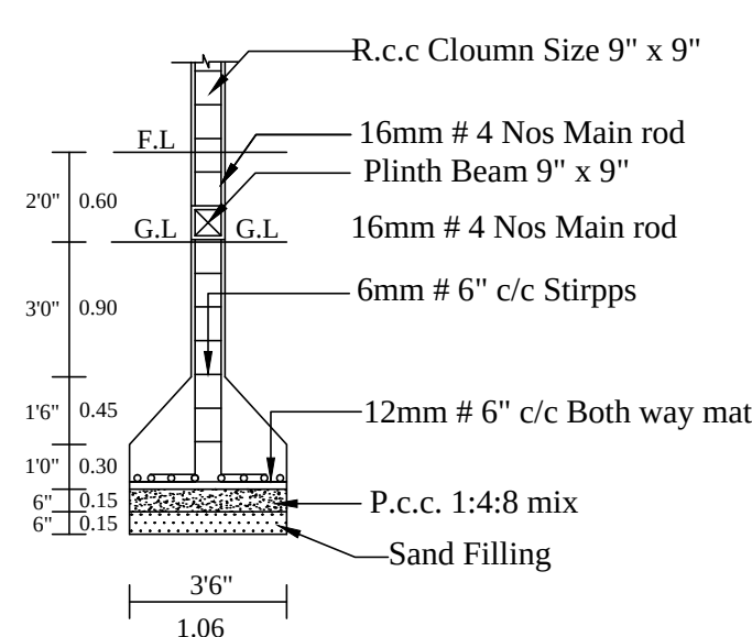
COLUMN DETIAL
