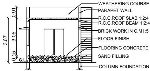
SECTION ON SS
