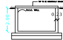
SECTION (SAMPLE)
