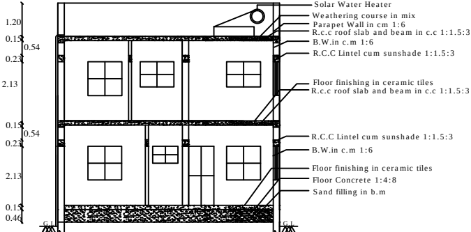
SECTION - "AB "
