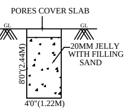
RAINWATER HARVESTING
