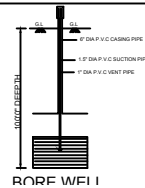
FRONT ELEVATION
