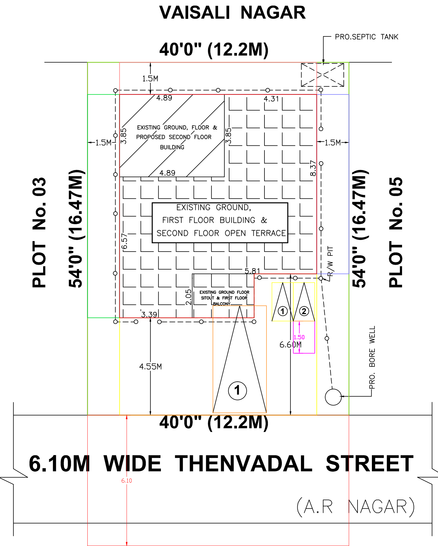
SITE PLAN
