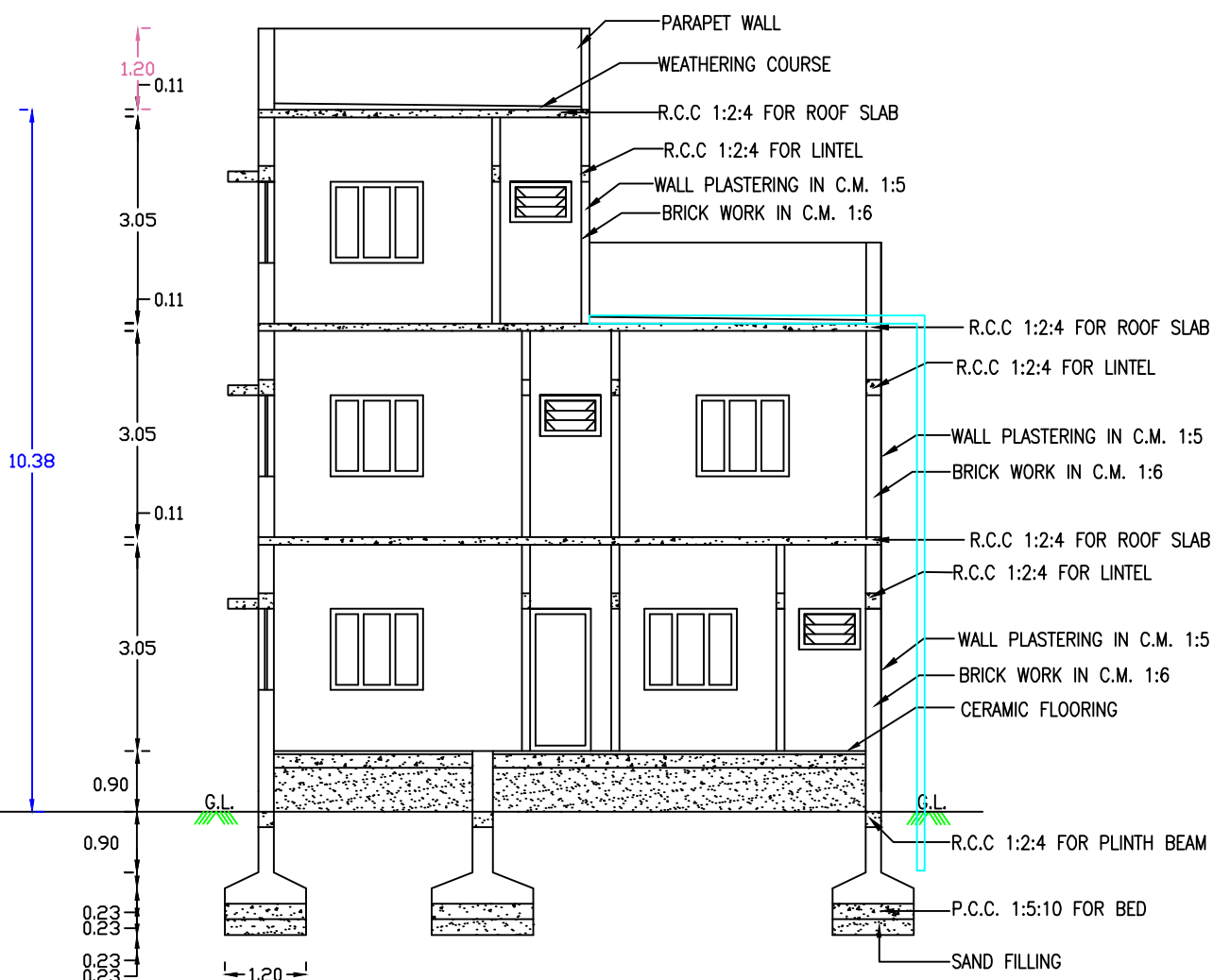
SECTION ON "RC"
