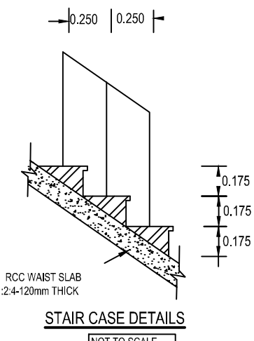
STAIR CASE DETAILS
