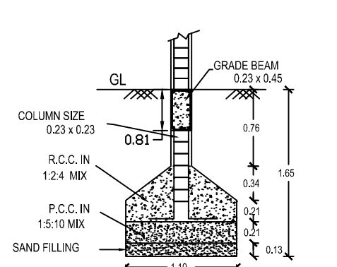
COLUMN DETAILS
